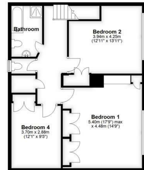
First Floor Approx. 71.7 sq. metres (772.3 sq. feet)
